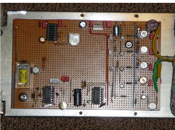
Abbildung 7: the control- board
