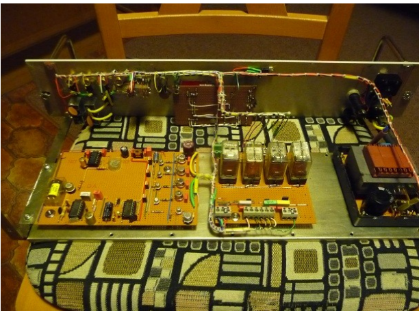
Abbildung 5: backview of the finished unit
