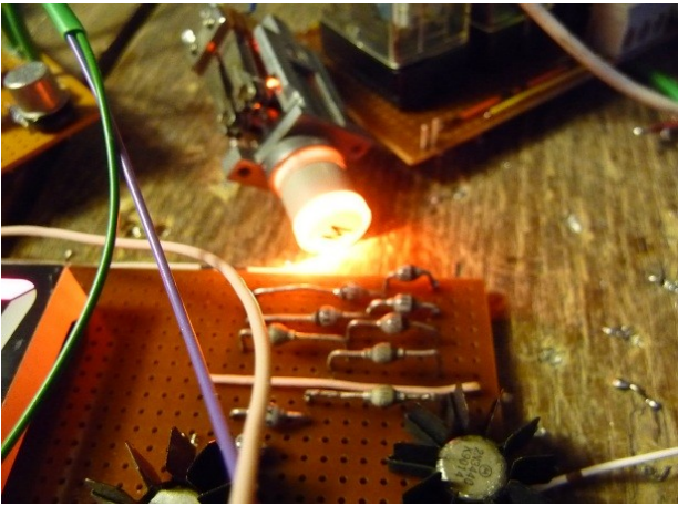
Abbildung 3: a flesh-LED indicates high vswr
