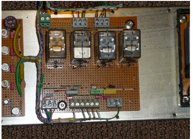
Abbildung 8: the relay- board
